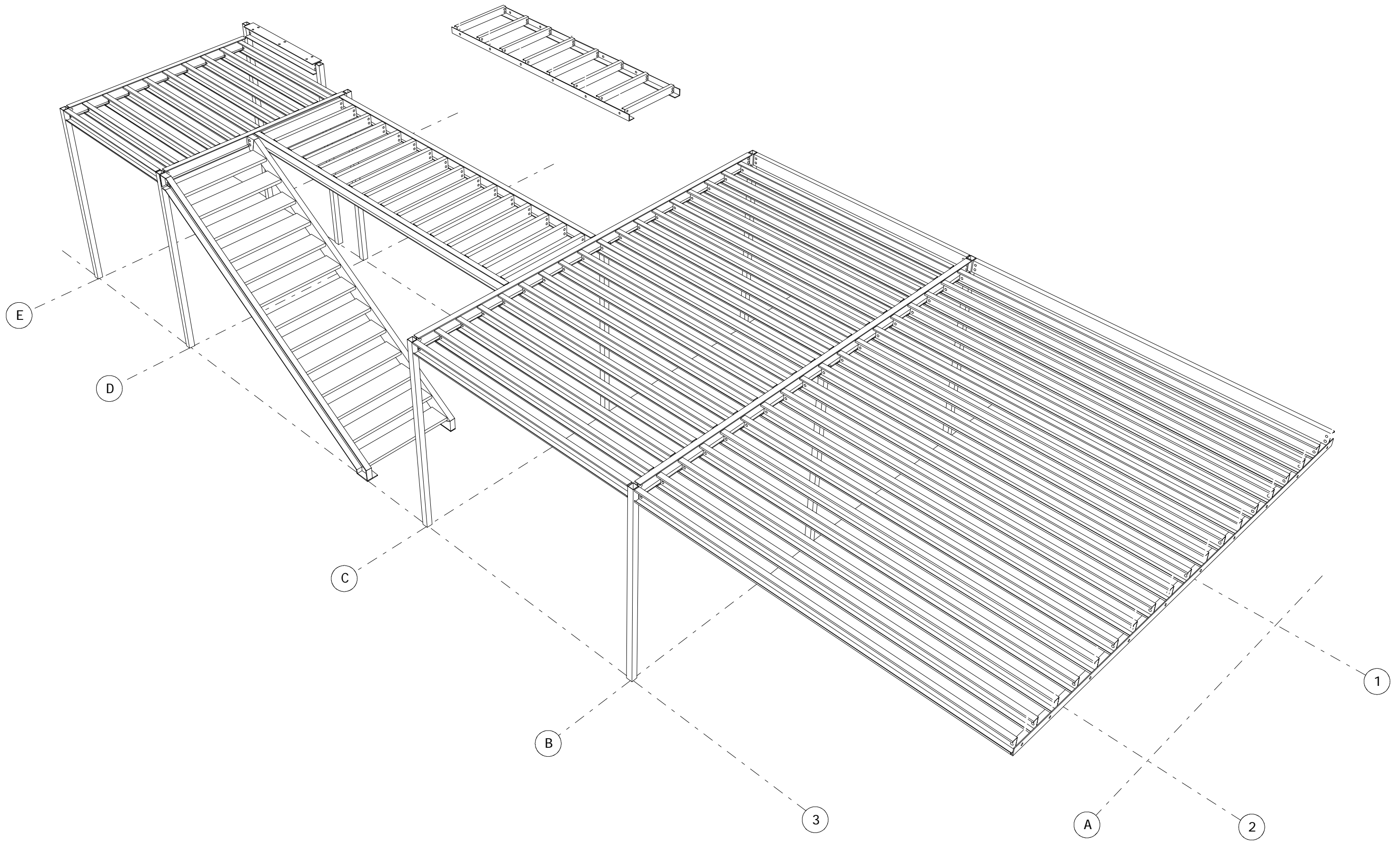
3-D VIEW
